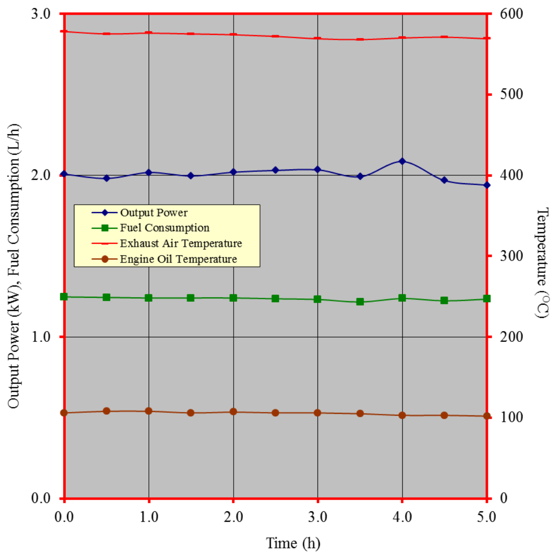
Figure 4. Performance characteristic curves during the continuous running test of the HONDA GX200 MEGA MARINE gasoline engine
