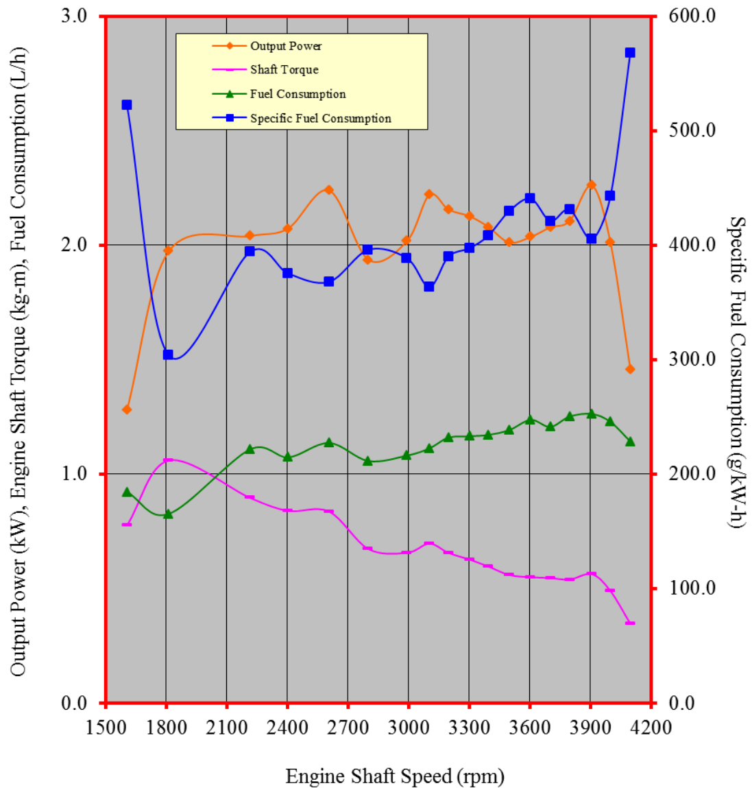
Figure 3. Performance characteristic curves of the HONDA GX200 MEGA MARINE gasoline engine
