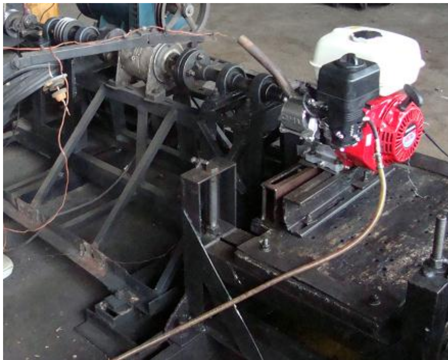
Figure 2. Test set-up of the HONDA GX200 MEGA MARINE Gasoline Engine.
